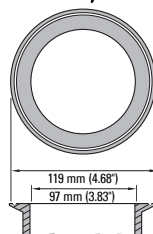
4" Sanitary Ferrule
